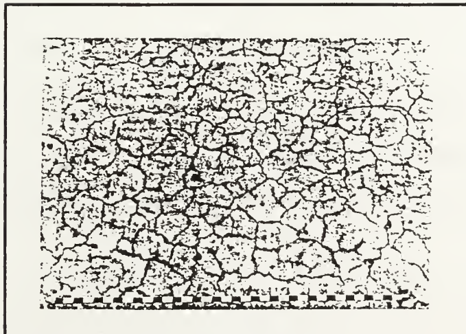
Figure 2.2 Map Cracking (Reference 4)
